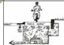
Porous, Raised Bike Lane
